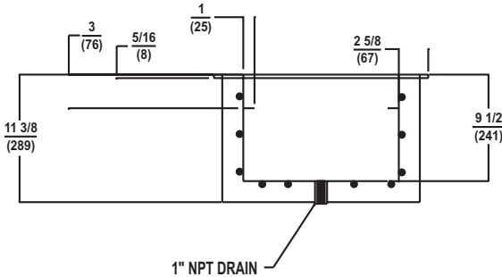
CROSS-SECTION OF COLD PAN
