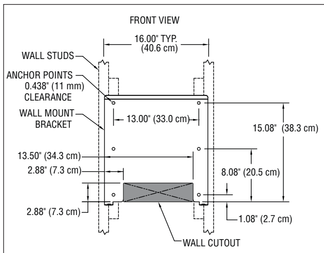
Fig. 5 – Wall-mount dimensions
